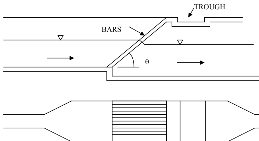
Figure 14.1 Bar Screen
