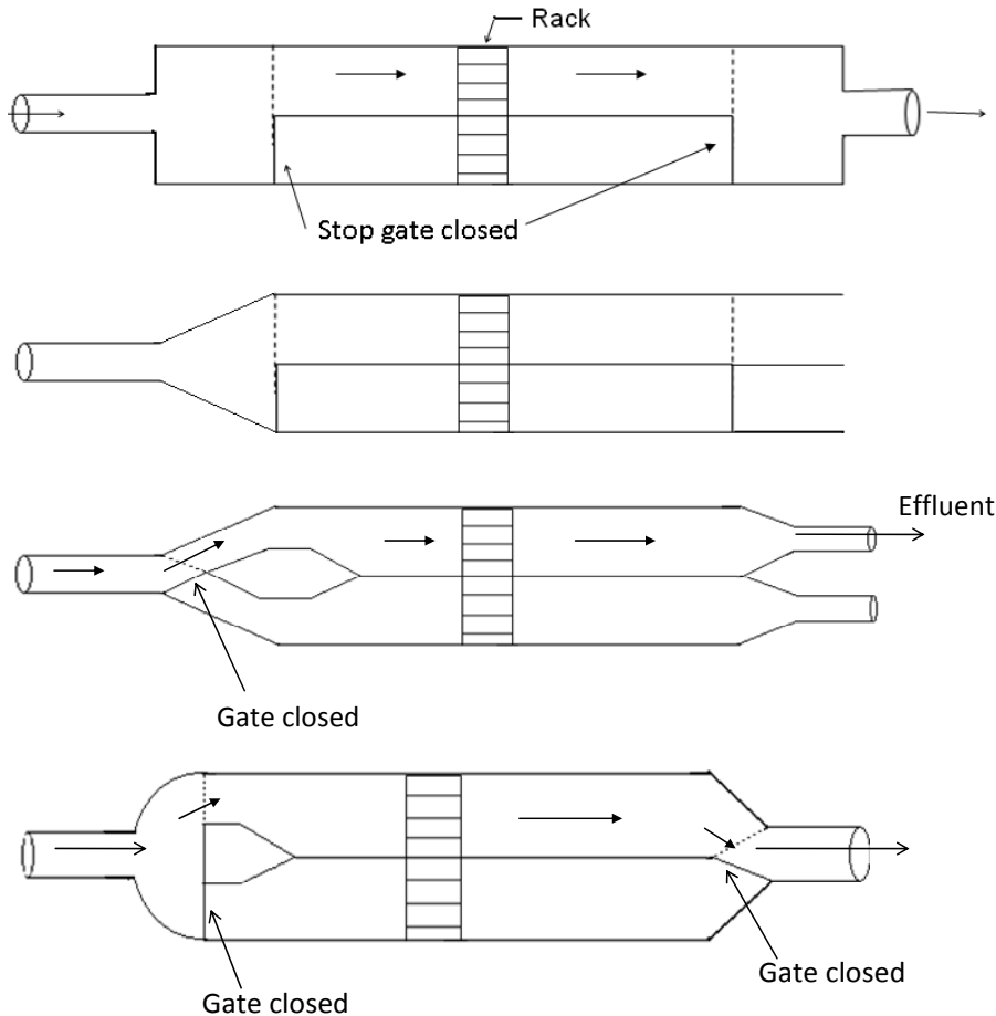
Figure 14.2 Double chamber bar screen and influent and effluent arrangement
