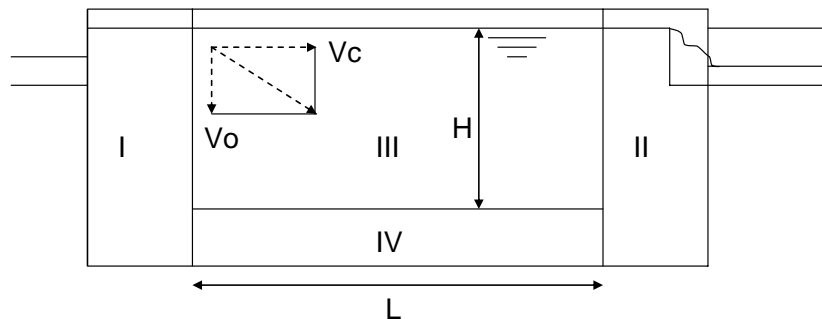
Figure 15.1 Compartments of grit chamber
