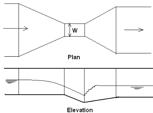
Figure 15.4 Parshall flume
