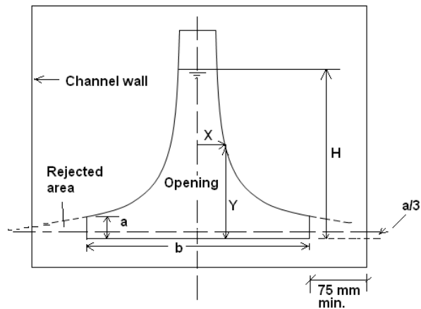
Figure 15.3. Proportional Weir
